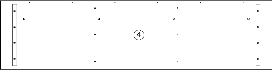
1627x414x41mm
