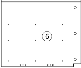
495x414x16mm
